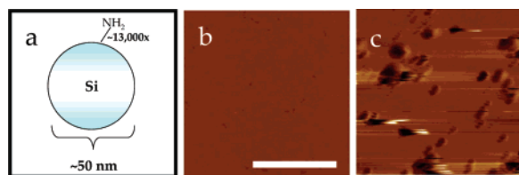
Figure 6. 50 nm amine coated silica spheres ( \sim 13,000 \text{NH}_2 /sphere) (a) were introduced onto a DMPC lipid bilayer (b) yielding a final concentration \sim 3 mg/mL (30 nM) of the silica spheres. The addition of the positively charged spheres resulted in the formation of circular defects on the bilayer ranging from 20 to 150 nm in diameter (c). The formation of new holes within the bilayer is similar to what is seen with G7- \text{NH}_2 PAMAM dendrimers. Scale bar is 500 nm.
